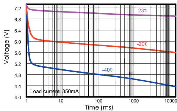
2. 2UPC1520 350mA Discharge Curve
